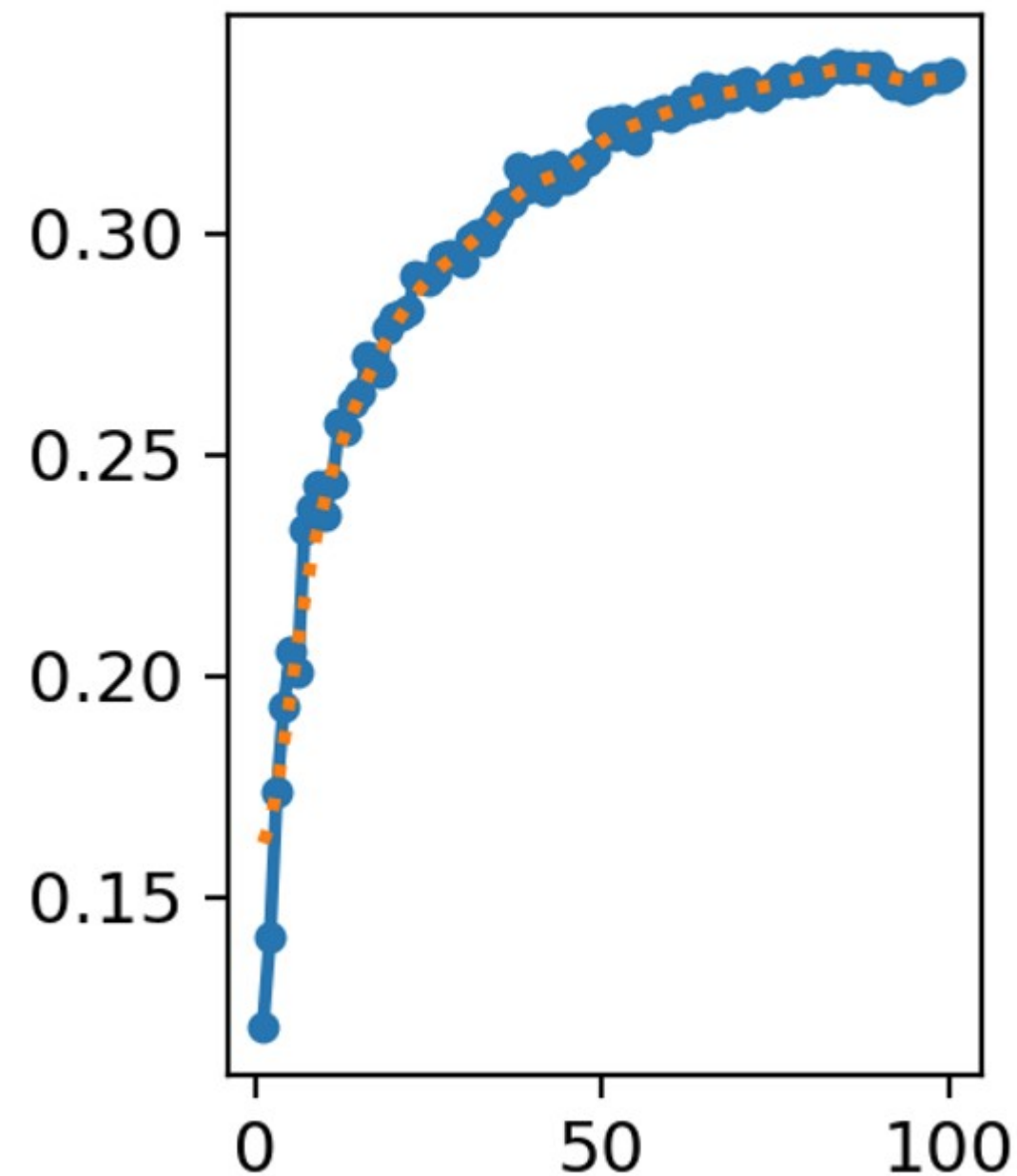
metrics/mAP50(B)
